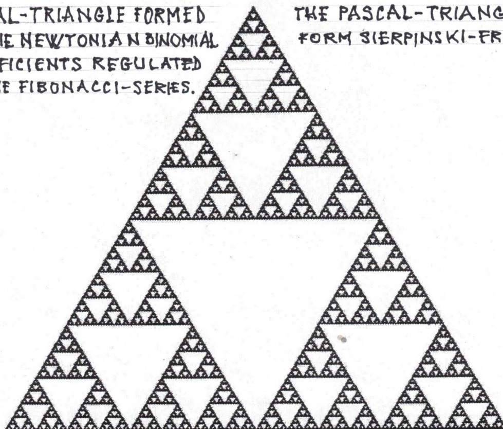
Figure (04.1) – Pascal-Fibonacci-Sierpinski Triangle
